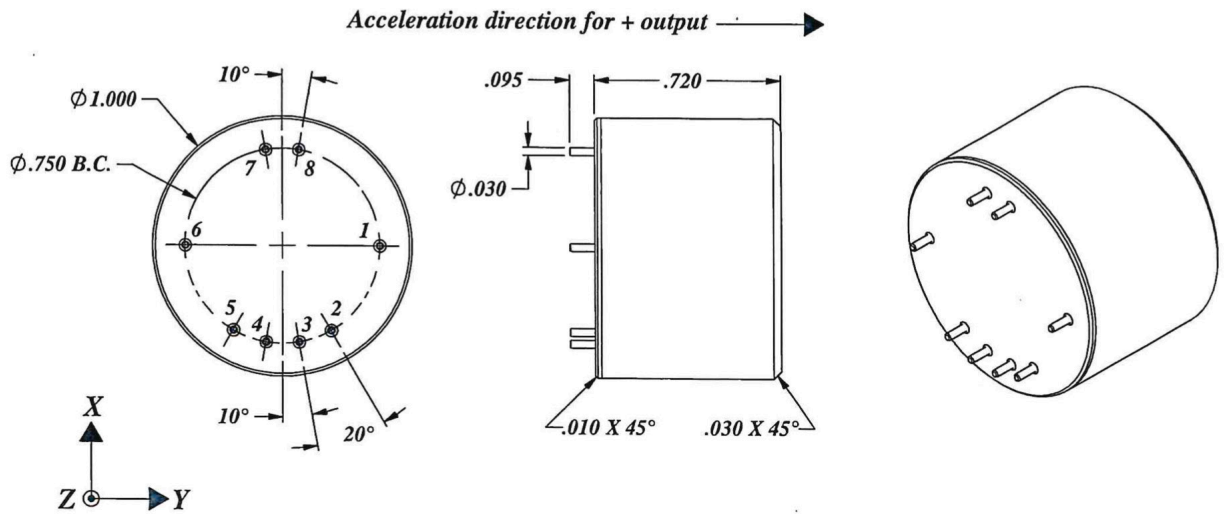
Figure 1. Model 80 MiniAcc Accelerometer
