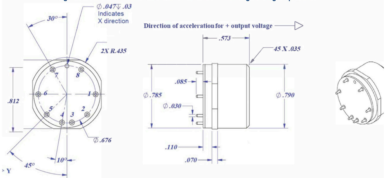
Figure 2. Model 60 MicroAcc Accelerometer - Package Design Option B
