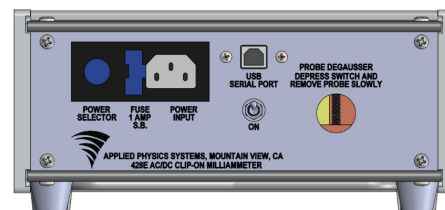
REAR PANEL
